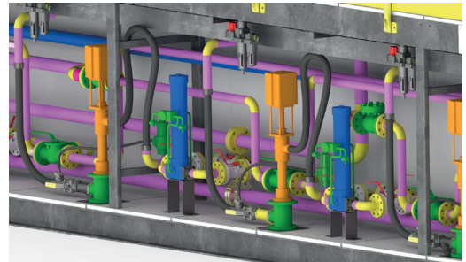
IN-CONTEXT PIPING ARRANGEMENT
