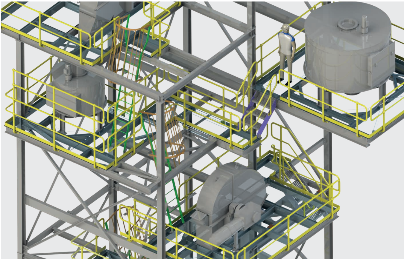
STAIRWAYS AND LADDERS CONNECTING PLATFORMS ON DIFFERENT LEVELS
