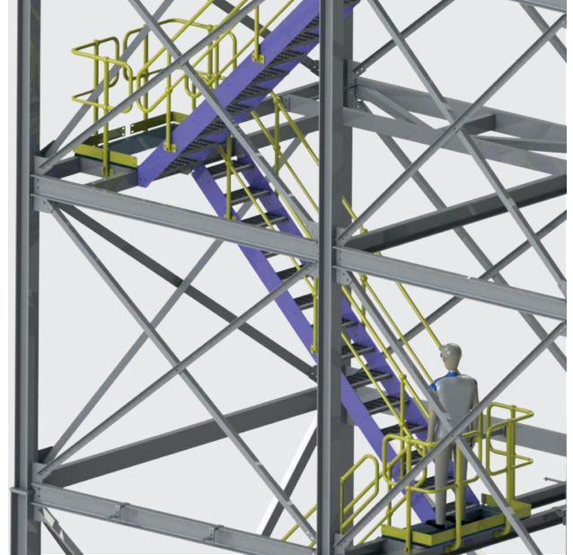
FLIGHTS OF STAIRS TO GAIN ACCESS TO TOP OF STRUCTURE
