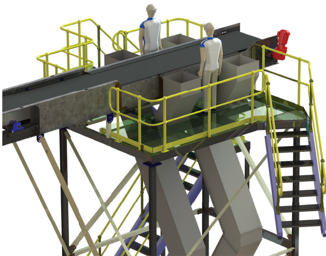
PICKING PLATFORM
